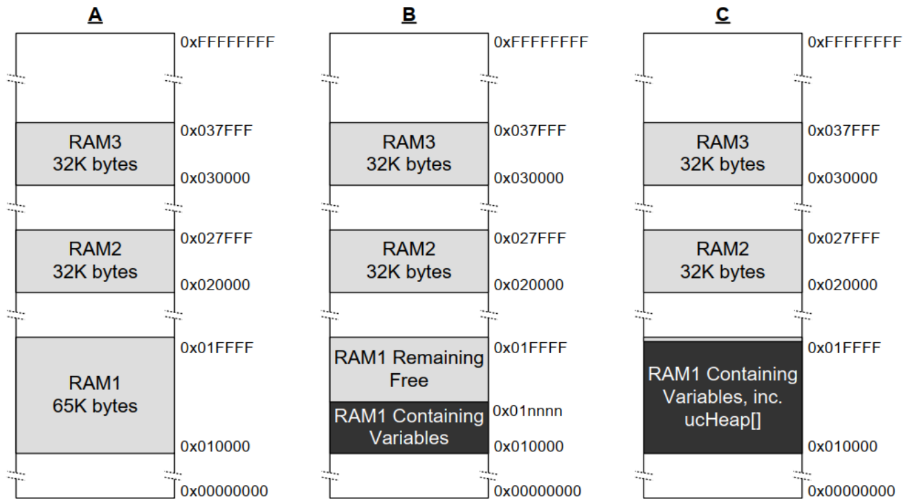
Figure 3.4 Memory Map
