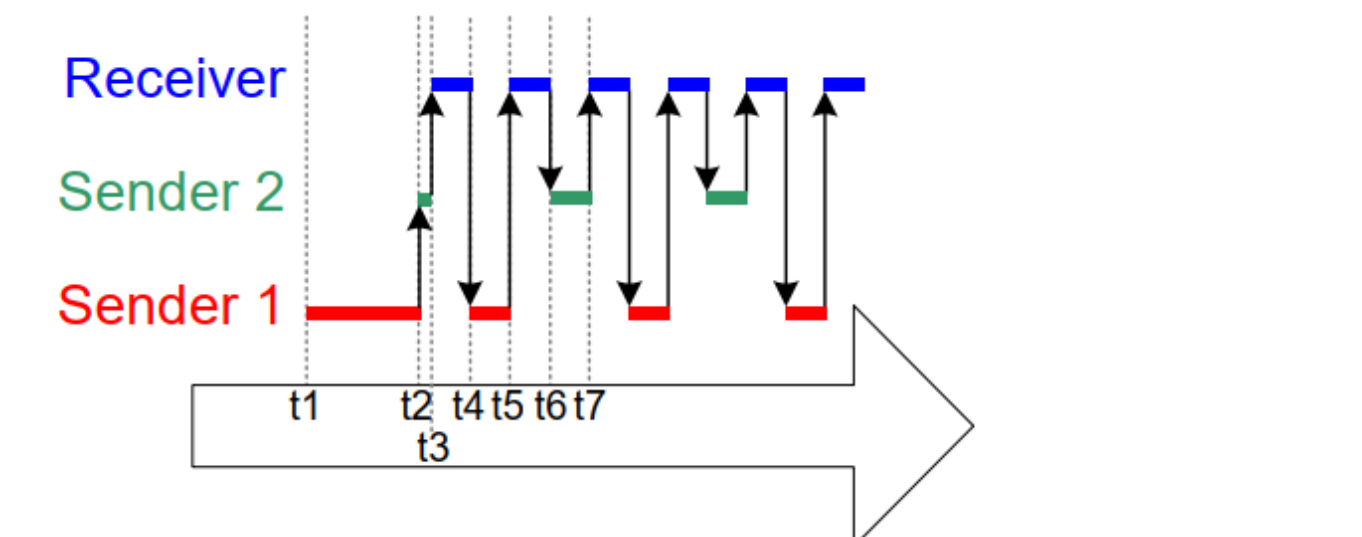
Figure 5.6 The sequence of execution produced by Example 5.2
