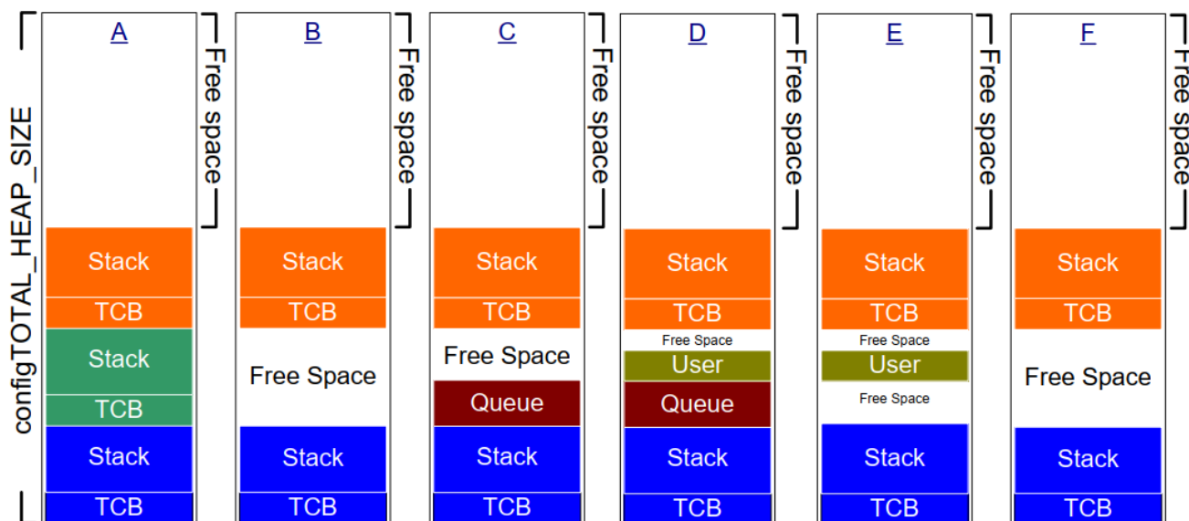
Figure 3.3 RAM being allocated and freed from the heap_4 array
