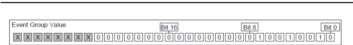
Figure 9.2 An event group in which only bits 1, 4 and 7 are set, and all the other event flags are clear, making the event group's value 0x92
